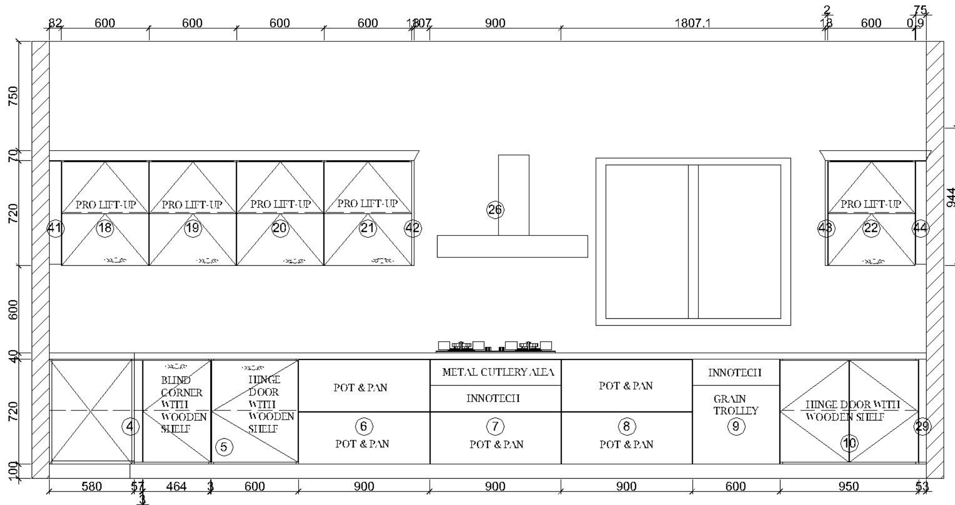
A View elevation drawing
