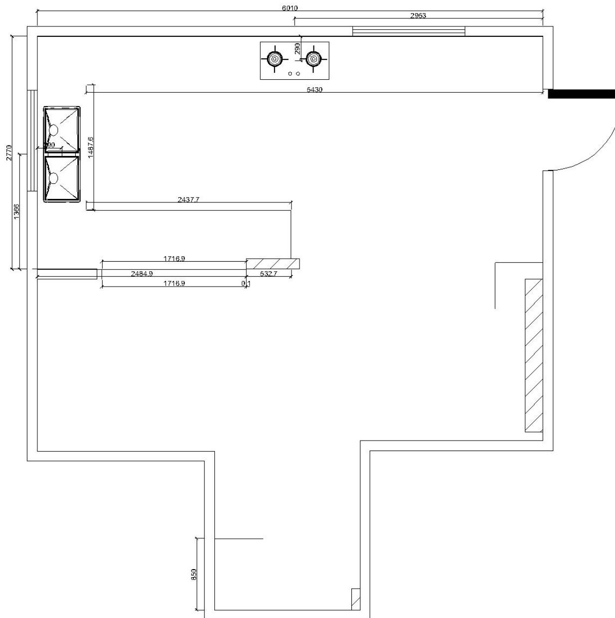
Worktop plan drawing
