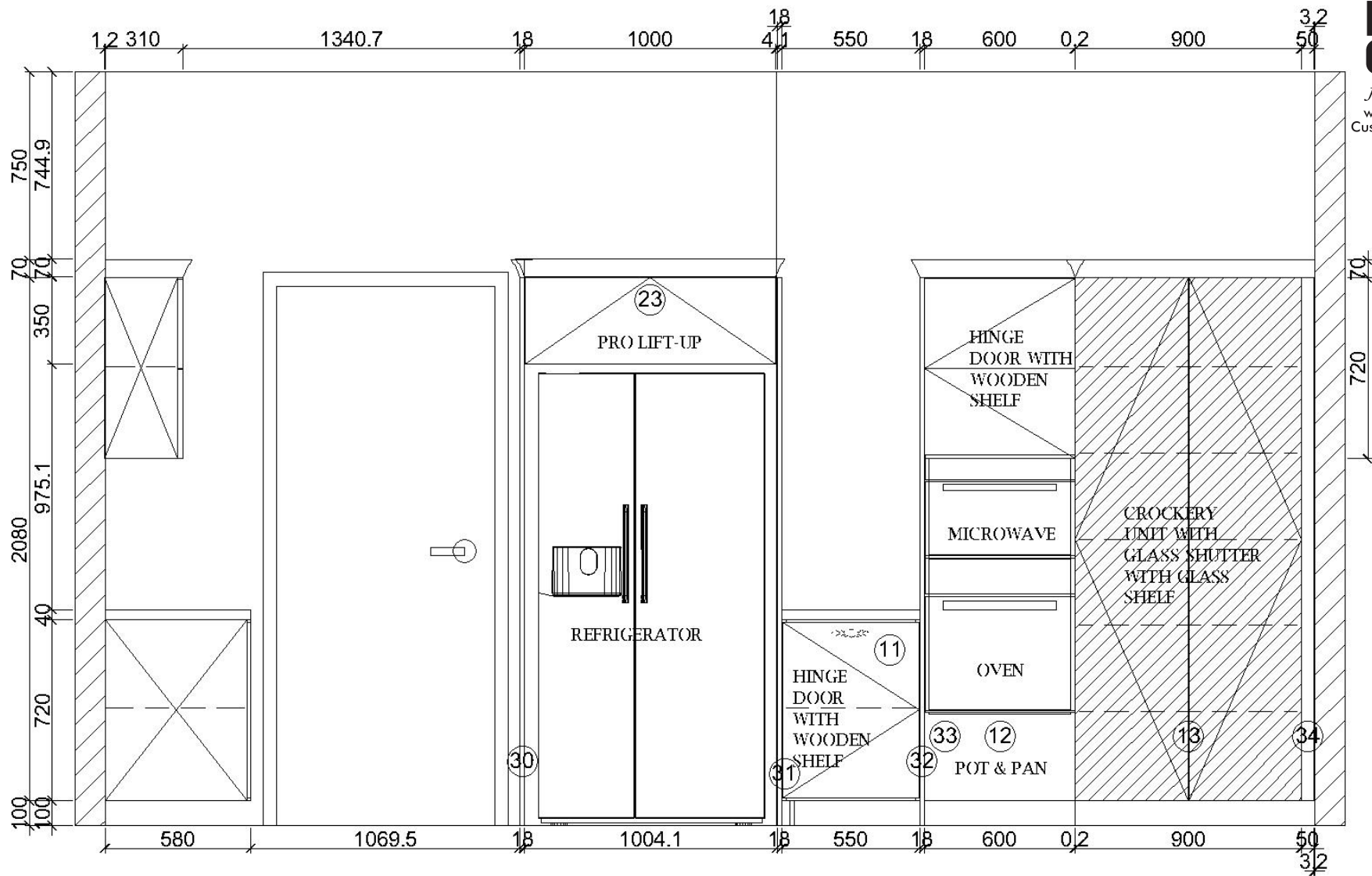
B View elevation drawing
