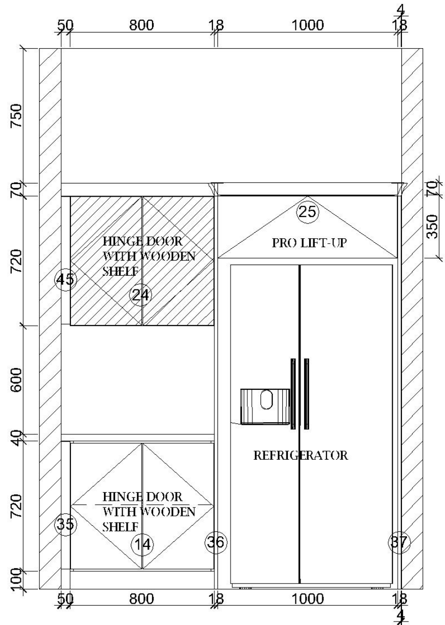
C View elevation drawing
