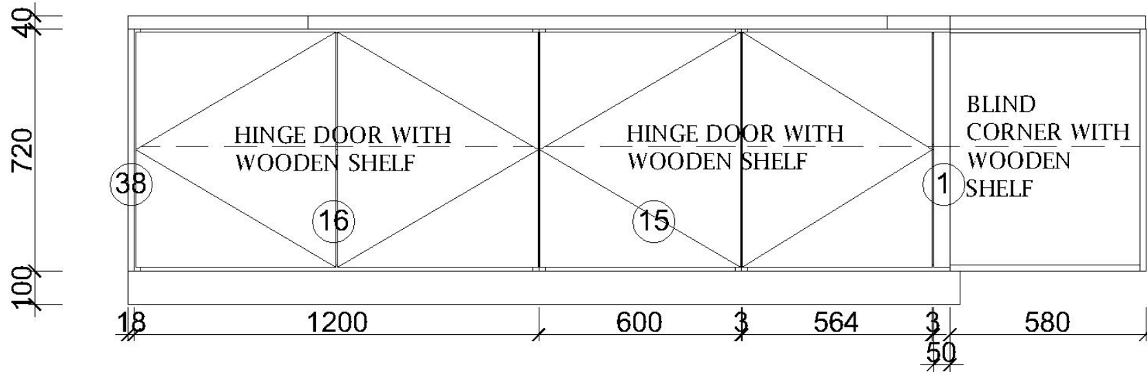
F View elevation drawing
